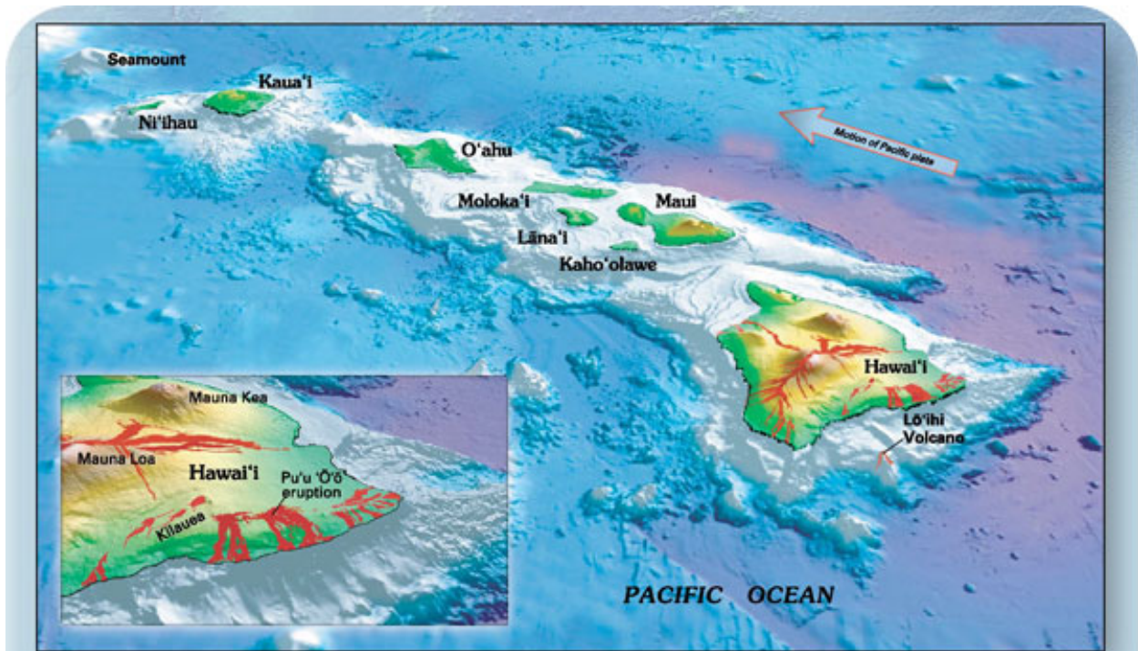
Figure 2. —Oblique view of the principal Hawaiian Islands and (the still submarine) Lō'ihi Volcano. Inset gives a closer view of the five volcanoes that form the Island of Hawai'i (historical lava flows are shown in red). The longest duration historical eruption on Kilauea's east-rift zone at Pu'u 'Ō'ō (inset), which began in January 1983, continues unabated (as of spring 2006). View prepared by Joel E. Robinson (USGS).
